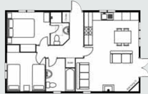
2 Bedroom, 2 Bathroom Lodge 32' x 20' (9.9m x 6.1m)
